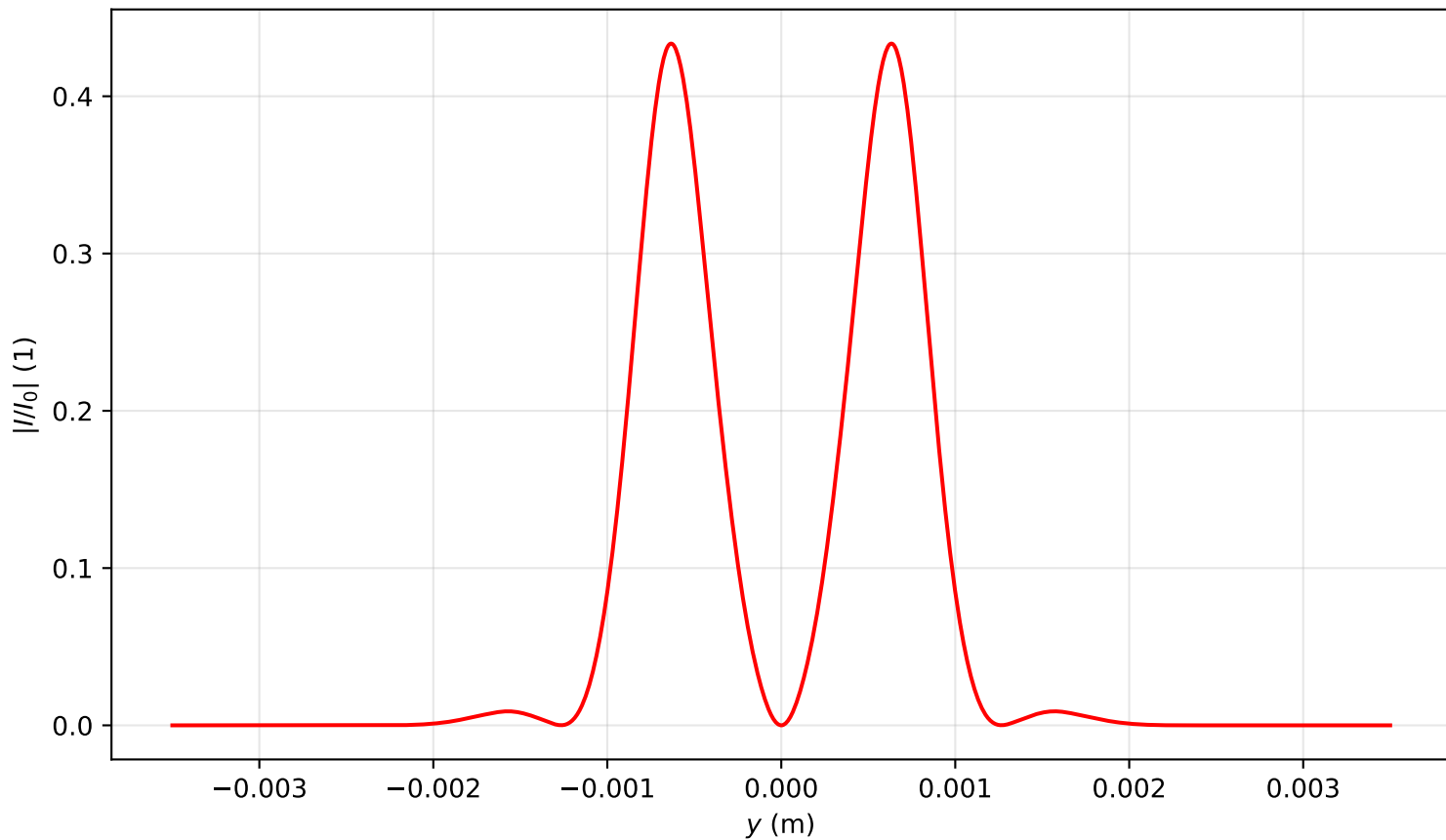
Intensity profile I(x=0, y, z=1.433)/I_0 , P_{in}=5.0P_{cr} , artificial time
